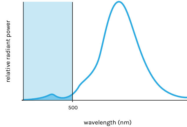
1800 K LED
