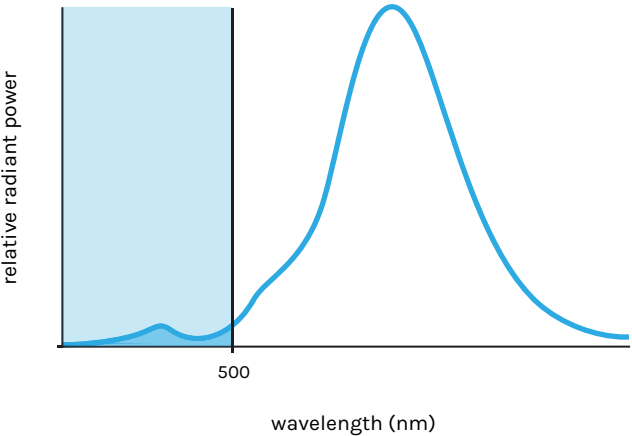
1800 K LED
