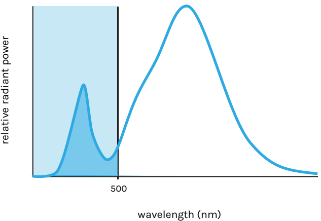
3000 K LED
