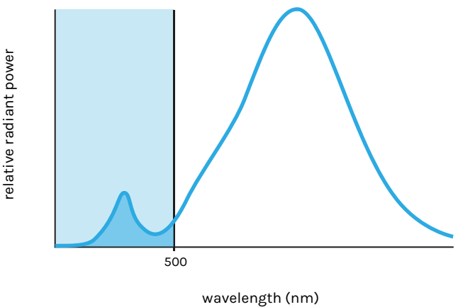
2200 K LED
